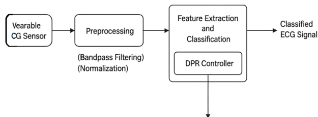
Fig. 2: FPGA-Based Real-Time ECG Classification System Architecture
