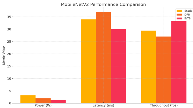
Fig. 7: MobileNetV2 Performance Comparison Under Static, DPR, and INT8 Configurations
