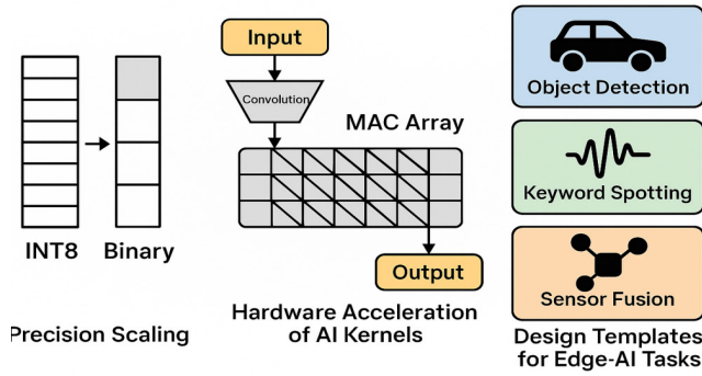
Fig. 6: Precision Scaling, Hardware Acceleration, and Task-Specific Design Templates for Edge-AI Optimization
