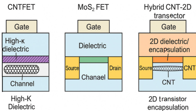
Fig. 2: Device schematic of CNTFET, MoS 2 FET, and hybrid CNT-2D heterostructure transistors, showing gate stack, channel, dielectric, and contact layers.
