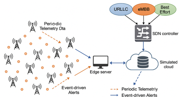
Fig. 4: NS-3-Based Simulation Setup of 5G-Enabled WSN Architecture for Industrial IoT with Edge Aggregation, mmWave Backhaul, and Network Slicing
