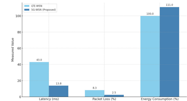
Fig. 7: Comparative Performance Analysis of LTE-WSN and 5G-Enabled WSN Architectures across Latency, Packet Loss, and Energy Consumption Metrics.
