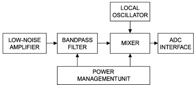
Fig. 3: Detailed Block-Level Architecture of the UWB RF Front-End
