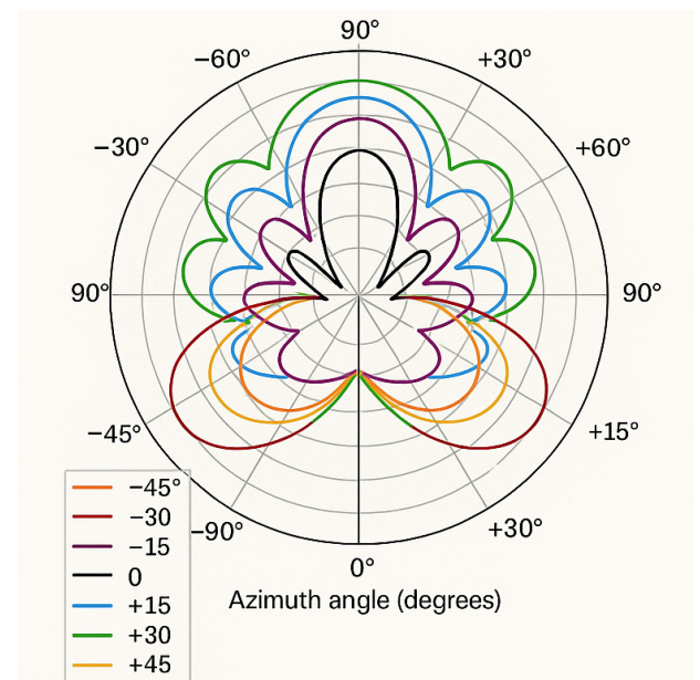
Fig. 2: Polar Plot of Radiation Patterns at Different Beam Angles
