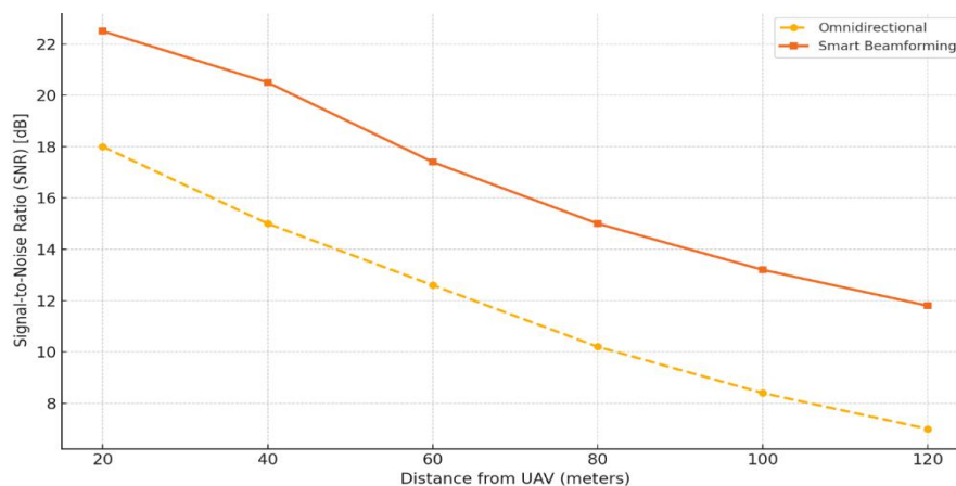
Figure 7. SNR vs. Distance for Omnidirectional vs. Beamforming Systems
