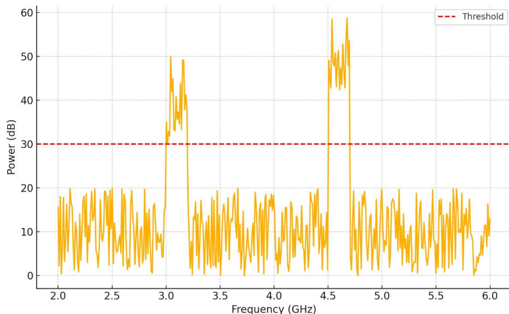
Fig 4. Spectrum Sensing and Decision Engine (FFT-Based Visualization)
