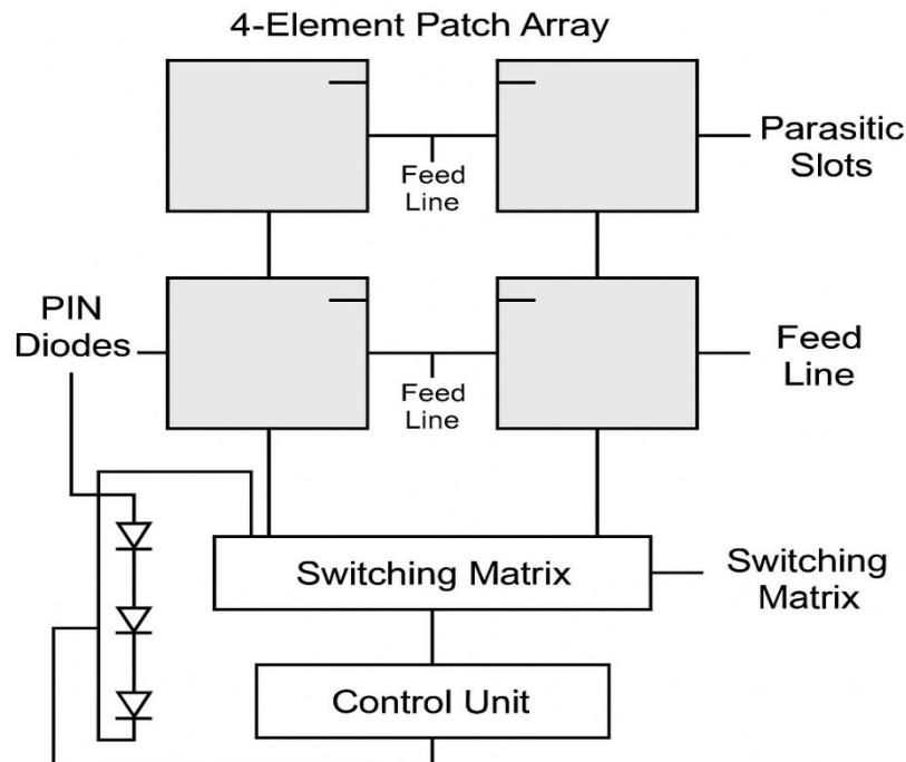
Fig 1. proposed reconfigurable antenna array system
