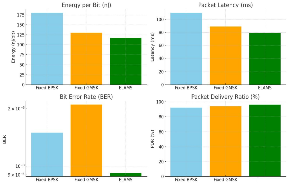
Figure 4. Performance Comparison of Modulation Schemes in Industrial WSN Simulation
