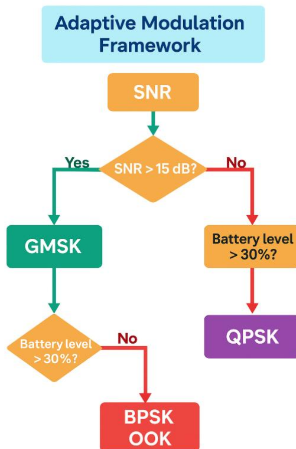
Figure 1. Adaptive Modulation Framework for Industrial Wireless Sensor Networks
