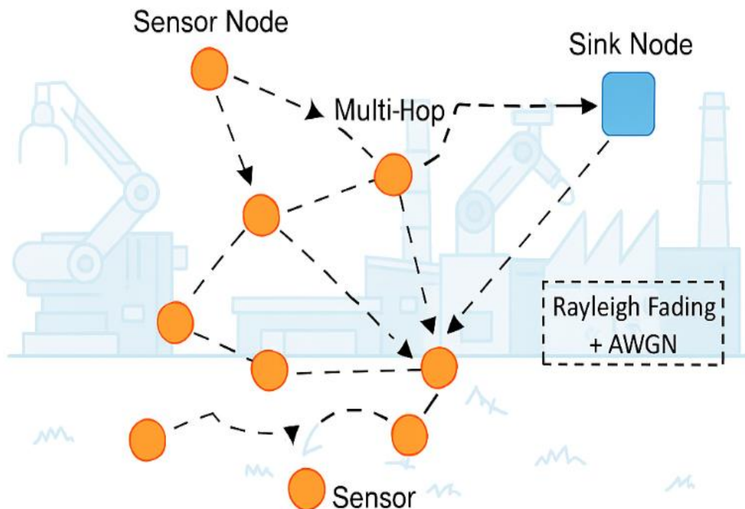
Figure 3. System Model of a Multi-Hop Wireless Sensor Network in an Industrial Environment
