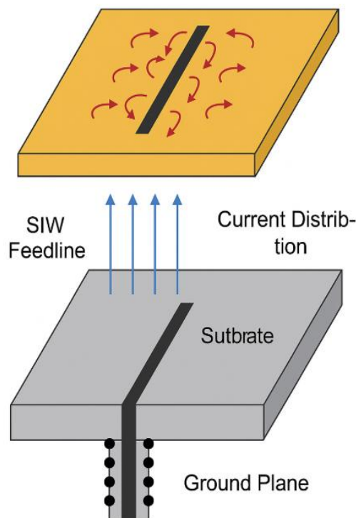
Figure 1. Exploded View of Slot-Loaded Microstrip Patch Antenna Element with SIW Feedline
