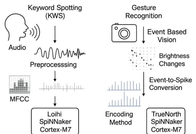
Fig. 3: Processing Pipeline for KWS and Gesture Recognition
