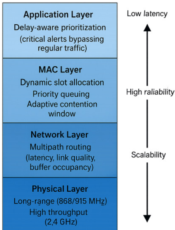
Fig. 3: Multi-Layer Protocol Stack for Low-Latency and Ultra-Reliable IoT Communication
