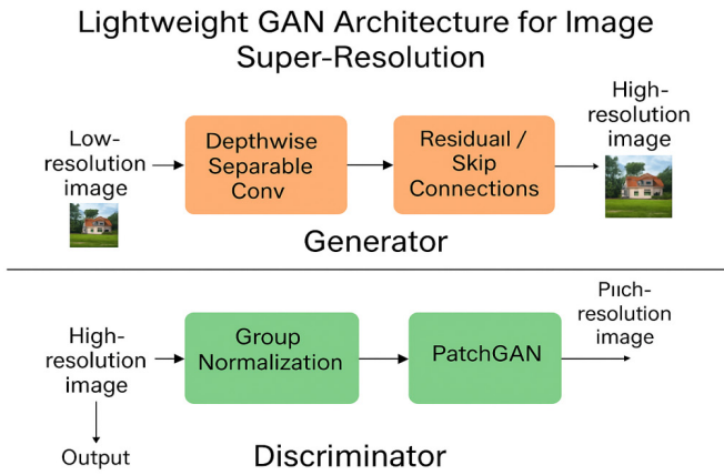
Fig. 1: Lightweight GAN Architecture for Image Super-Resolution
