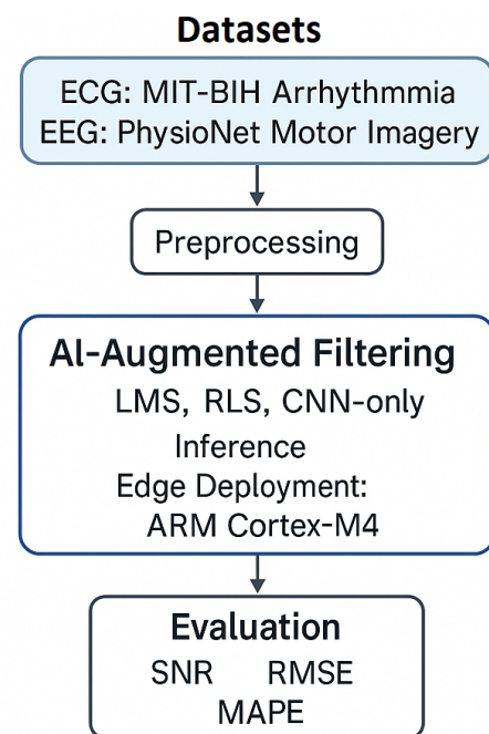
Fig. 3: Experimental Pipeline for AI-Augmented Adaptive Filtering Framework
